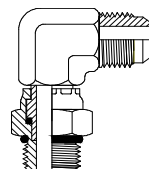
JIC Male UNO Male Swivel Page 82
