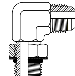
JIC Male Metric Stud Male Page 80
