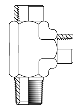
BSPT Female BSPT Male BSPT Female Page 103
