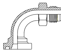
JIC Male Code 62 Flange Page 78
