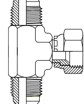
JIC Male JIC Male JIC Female Page 99
