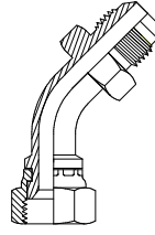
JIC Male JIC Female Page 68
