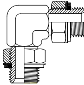
BSPP Adj Male BSPP Adj Male Page 76
