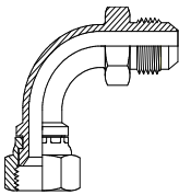
JIC Male JIC Female Page 86
