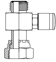
ORFSM x ORFS Swivel UNO Cross Port Page 108
