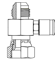
JICM x JIC Swivel BSPT Cross Port Page 109
