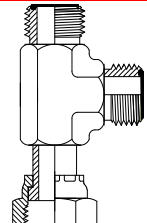
ORFS Male ORFS Female ORFS Male Page 100
