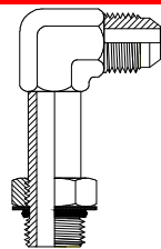
JIC Male UNO Male Page 81
