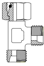
DKL Male DKOL Female DKL Male Page 143
