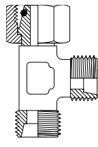
DKS Male DKOS Female DKS Male Page 143
