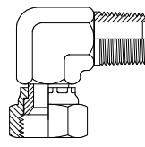
NPT Male JIC Female Page 87
