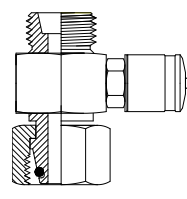
DKL M x DKOL Female BSPP Cross Port Page 107
