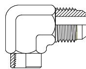
JIC Male NPT Female Page 90
