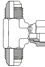
JIC Male JIC Male JIC Female Page 99
