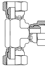
BSP Female BSP Female BSP Female Page 101
