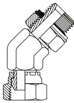
BSPP Male BSP Female Page 68
