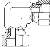
JIC Female JIC Female Page 90
