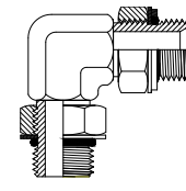
BSPP Adj Male UNO Male Page 76
