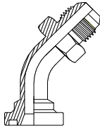
JIC Male Code 61 Flange Page 63
