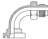
JIC Male Code 61 Flange Page 77
