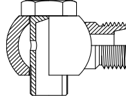
Metric DKL Male Banjo Page 125
