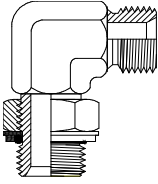
BSPP Male BSPP Adj Male Page 74
