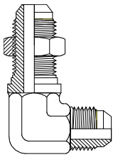
JIC Bulkhead Male JIC Male Page 92
