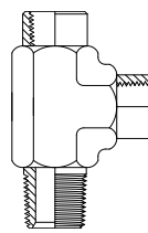
BSPT Female BSPT Male BSPT Female Page 103
