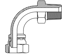
BSPT Male BSP Female Page 89
