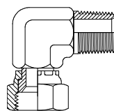
BSPT Male JIC Female Page 89
