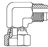
JIC Male JIC Female Page 86
