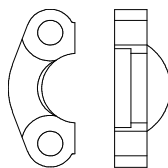
Code 62 Split Clamps Page 111
