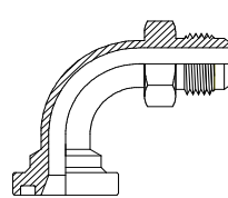
JIC Male Code 62 Flange Page 78
