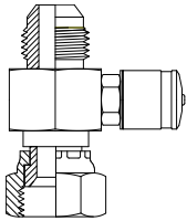
ORFSM x ORFS Swivel BSPP Cross Port Page 108
