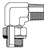
BSPT Male BSPP Adj Male Page 84
