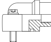
SAE Code 61 BSPP Fixed Female Page 114
