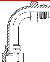
JIC Male JIC Female Page 86
