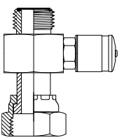
ORFSM x ORFS Swivel BSPT Cross Port Page 108
