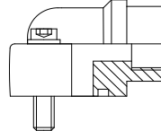
SAE Code 62 BSPP Fixed Female Page 114
