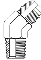
JIC Male BSPT Male Page 66
