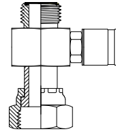
ORFSM x ORFS Swivel UNO Cross Port Page 108
