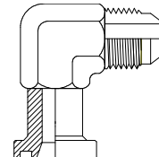
JIC Male Code 61 Flange Page 77
