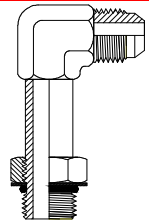
JIC Male UNO Male Page 81
