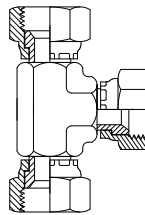
JIC Female JIC Female JIC Female Page 101
