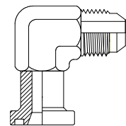
JIC Male Code 62 Flange Page 78
