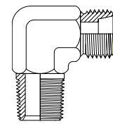
ORFS Male BSPT Male Page 132
