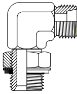
Metric DKL BSPP Adj Male Page 124
