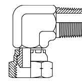
NPT Male NPSM Female Page 87
