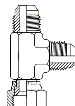
JIC Male JIC Female JIC Male Page 100
